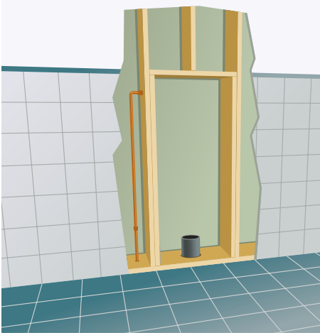
Route the drain and supply; prepare the wall studs.
