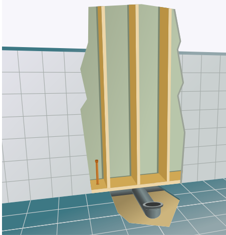
Open the wall and floor.
