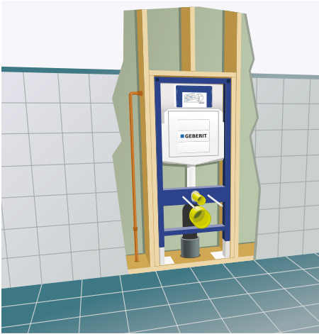
Install the tank and carrier.
